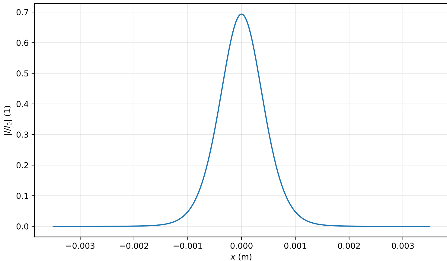
Intensity profile I(x, y = 0, z = 2.468m)/I_0 , P_{in}=0.5P_{cr} , artificial time
